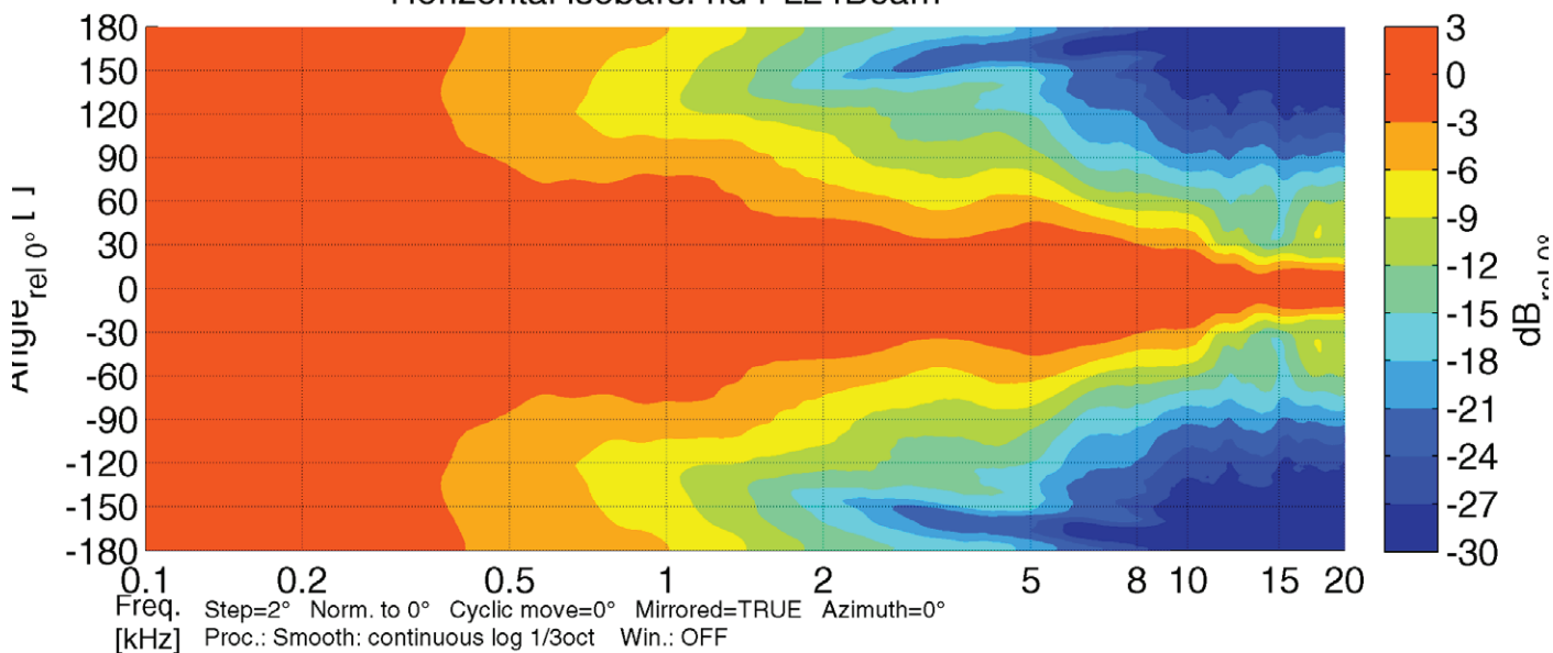
Horizontal isobars: hd PL24Beam
